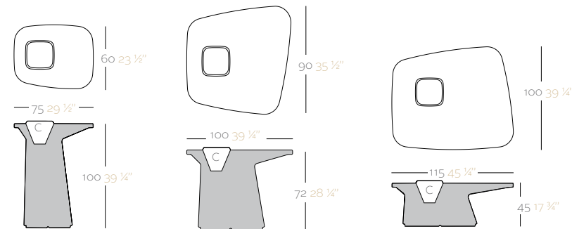
MOMA Table High MOMA Mesa High
