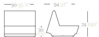
REST Sofa Central Unit REST Sofá Módulo Central
