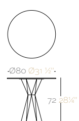
VERTEX Table Ø31 1/2" VERTEX Mesa Ø80
