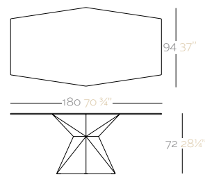
VERTEX Table 180 VERTEX Mesa 180
