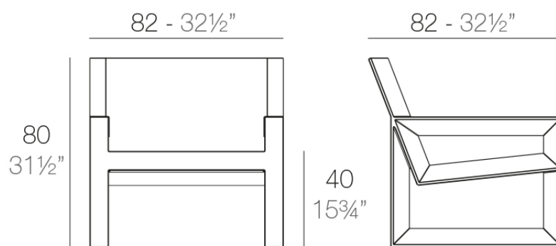
FRAME Butaca FRAME Lounge Chair
