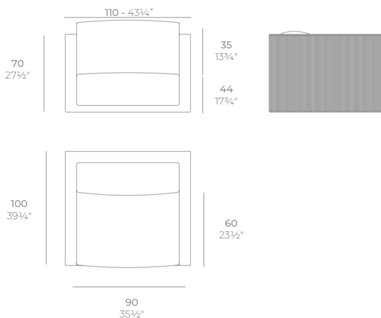
GATSBY Butaca GATSBY Armchair ref. 54403
