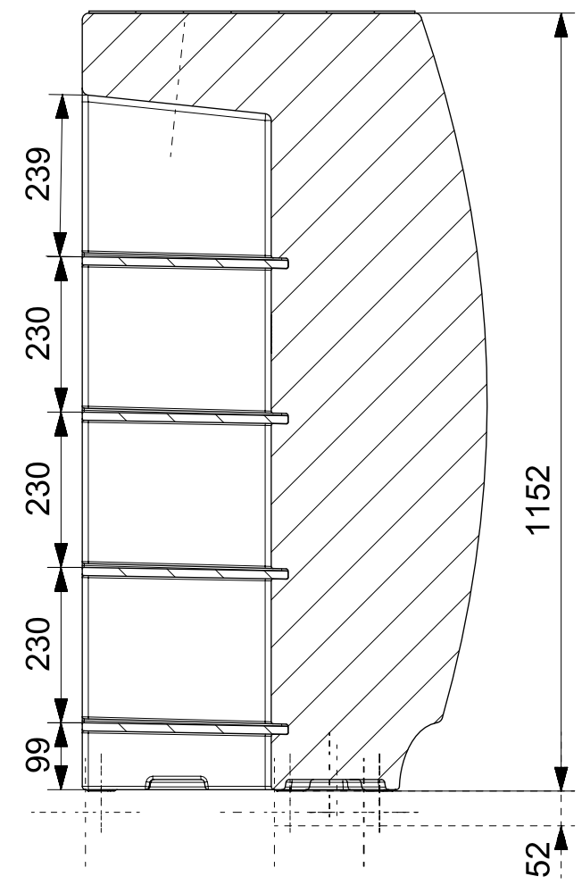
SECTION B-B
