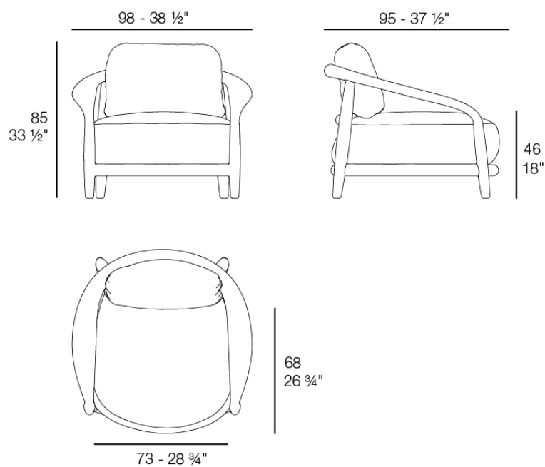
FUSTA Butaca FUSTA Armchair Ref. 54870
