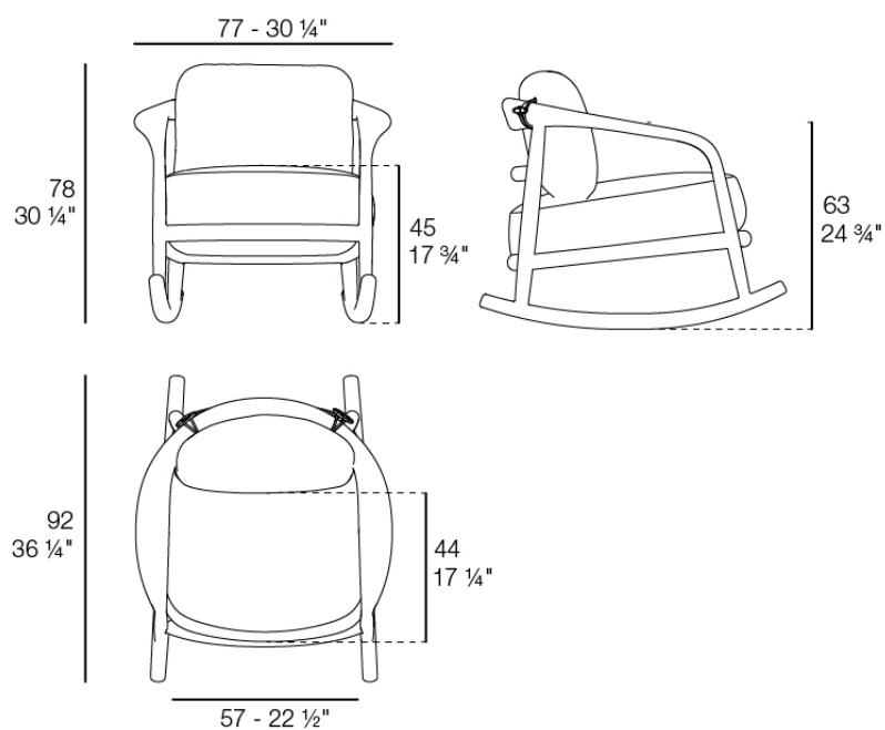
FUSTA Balancín FUSTA Rocking Chair Ref. 54877
